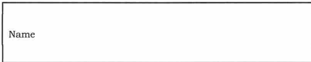
Swimlanes Pool
